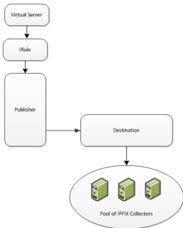
Figure 8: Association of logging configuration objects
